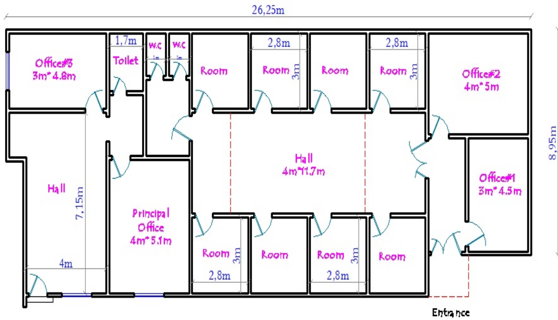
Ground floor plan for Topruk DC
